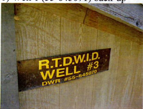
3 & 4) Well 3 (55-645070) pump house and insulated well head.
